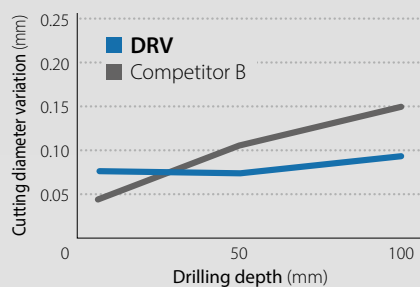
Comparison of cutting diameter variation (In-house evaluation)
